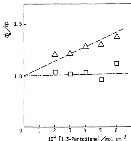
Fig. 8. Stern-Volmer plots for quenching of the photoreactions of 2-pyridinecarboxamide (1) by 1,3-pentadiene in the absence of sulfuric acid. [1]=9.9×10 -3 mol dm -3 ; irradiation time, 10 h. ---△---, methylation at the 5-position; ----□----, hydroxymethylation at the 4-position.
